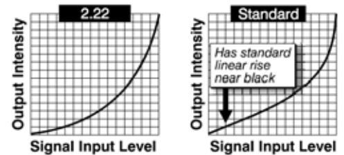
FIGURE 3-9 GAMMA CURVE
